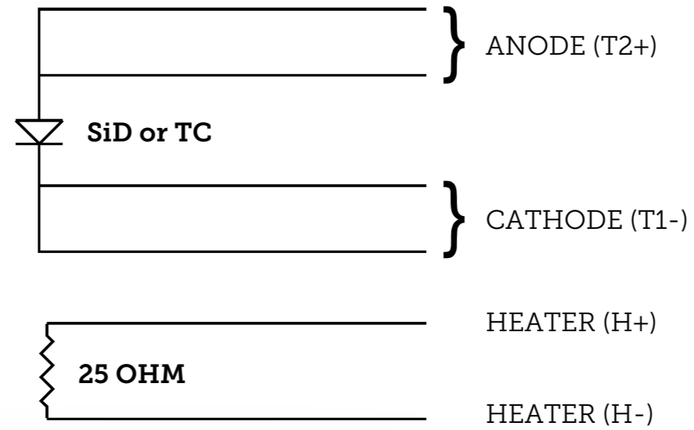
MK16 Pinout
