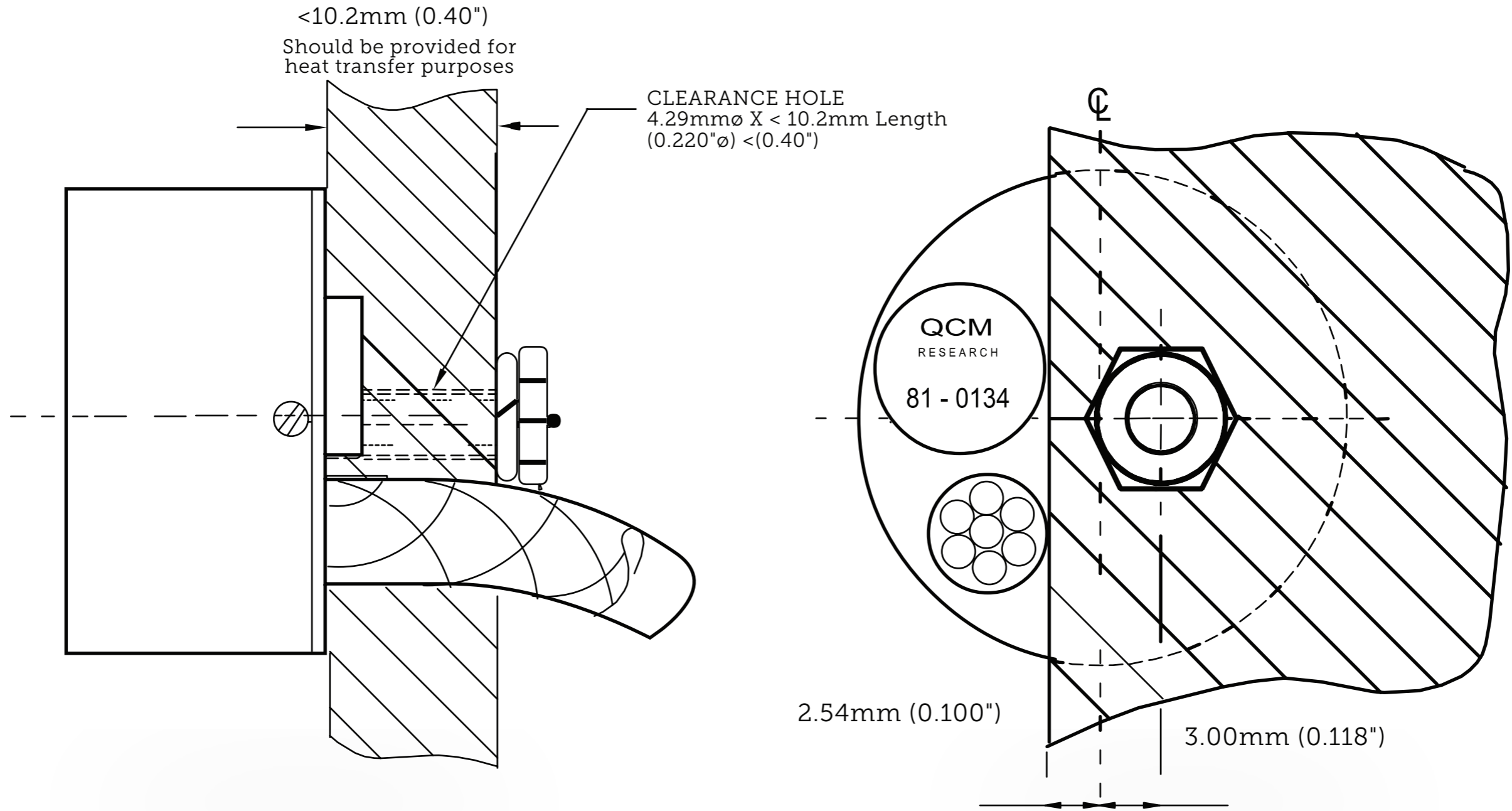
Heat Sink Partial Coverage
