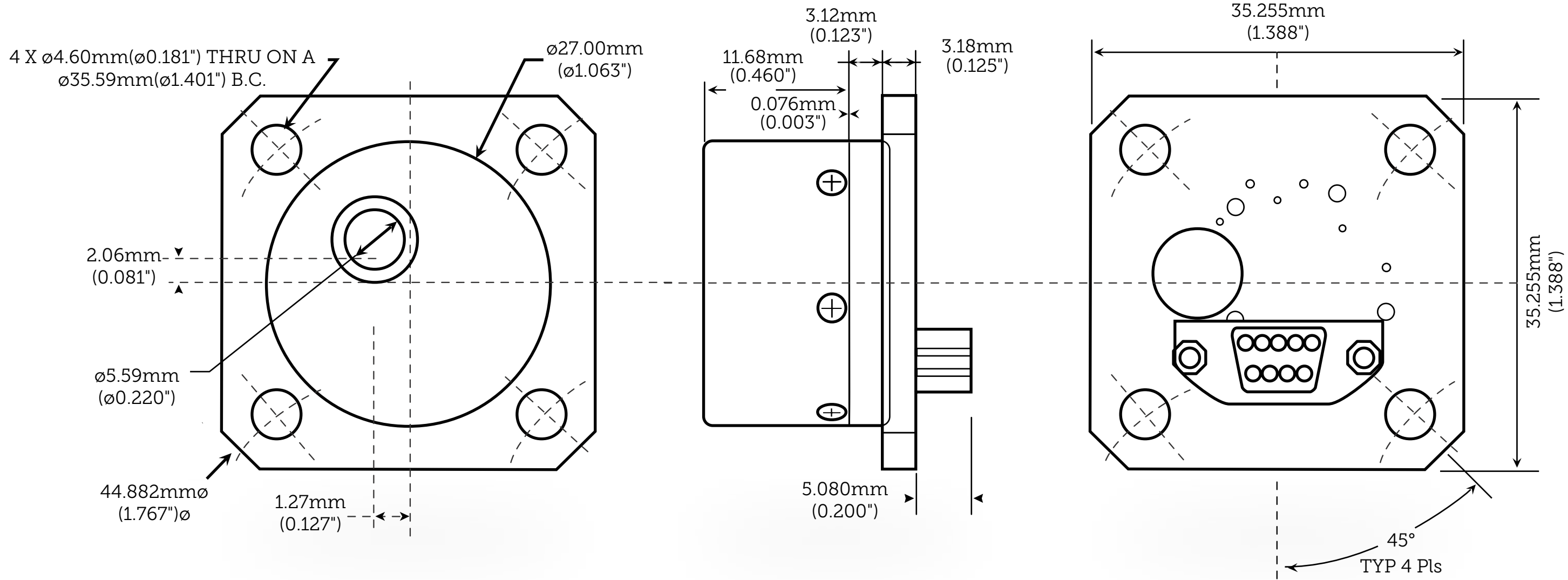
MK26-2 Dimensions
