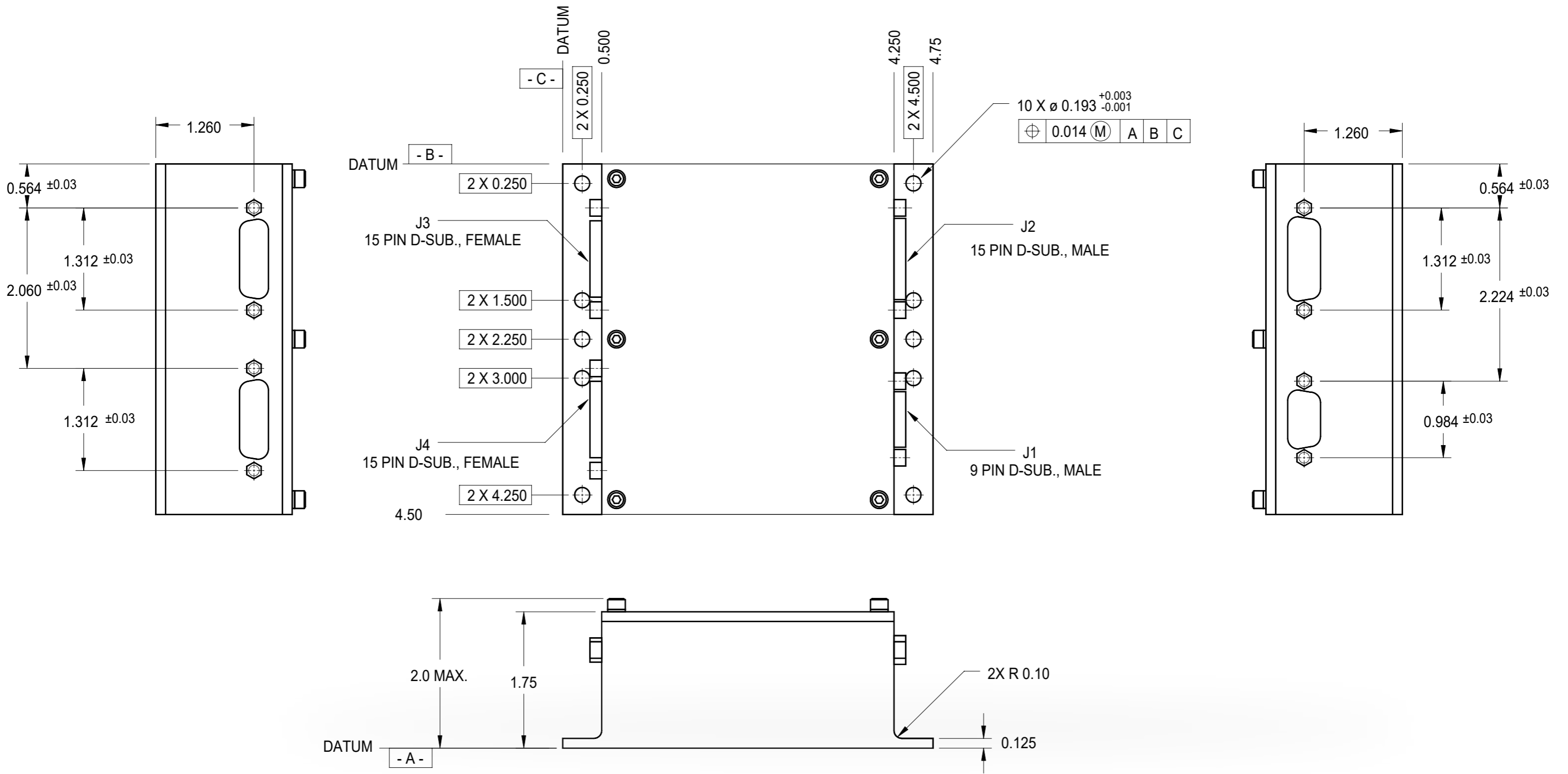
MODEL 3000 DIMENSIONS
