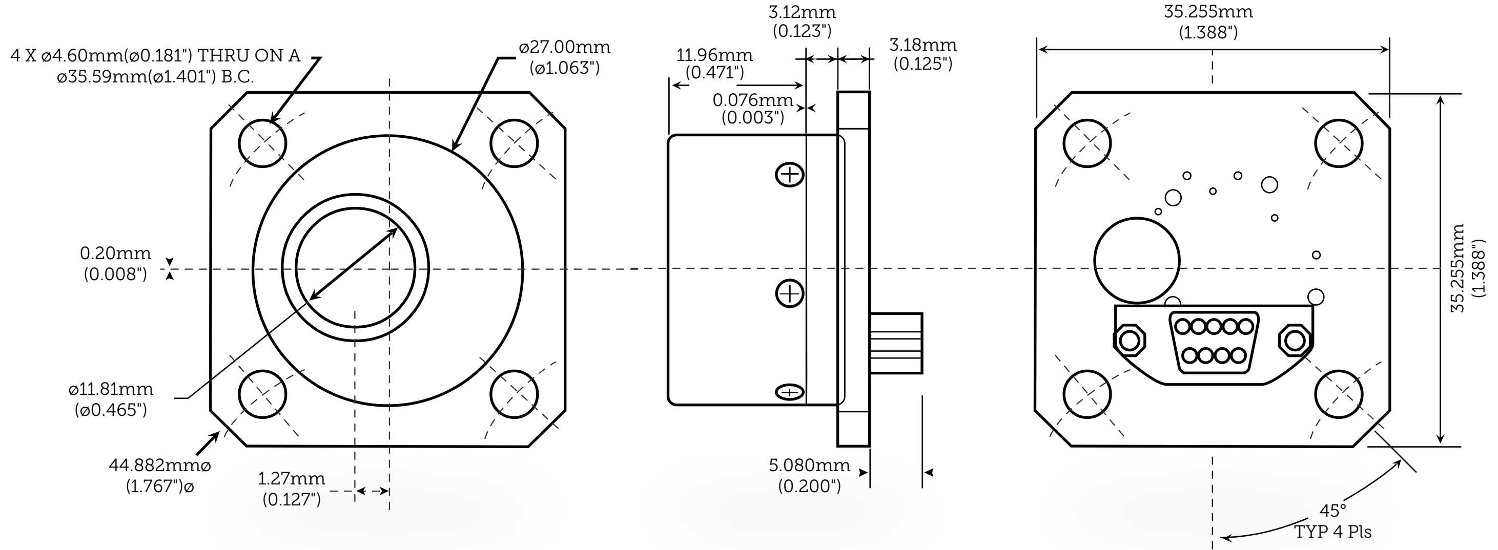
MK26-3 Dimensions
